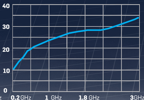
LP-02 - Antenna Factor
