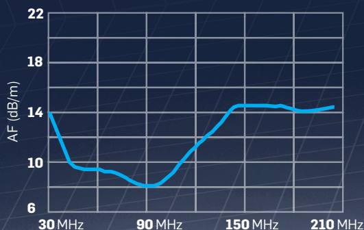
BC-01 - Antenna Factor
