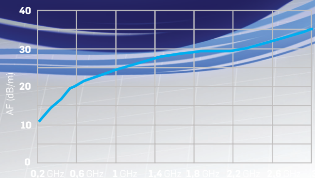
LP-02 - Antenna Factor @ 10m
