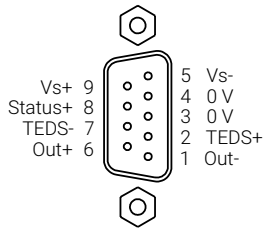
Figure 1: D-sub-9 female connection pinout
