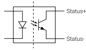
Figure 2: Status signal optocoupler
