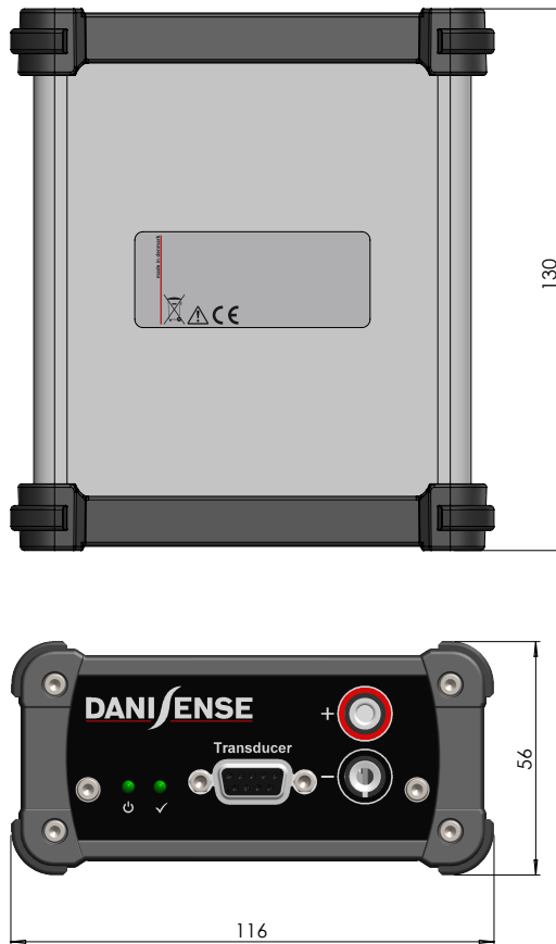
Figure 3: Box dimensions
